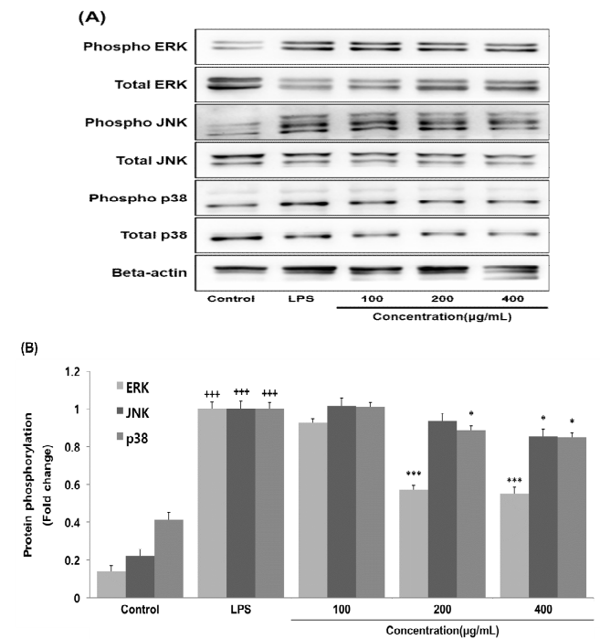
Fig. 5. Effects of HGC on protein phosphorylation level in RAW264.7 cells. RAW264.7 cells were treated by 100, 200 and 400 µg/mL of HGC with 500 ng/mL of LPS for 24 h. The protein phosphorylation level were measured using a western blot assay. The results were presented by the mean±standard error of mean from three independent experiments (Significance of results, +++ : p<0.001 compared to control, * ; p<0.05, *** ; p<0.001 compared to LPS). (A); protein phosphorylation level (B); graph image
