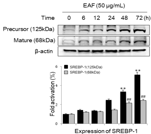
Fig. 6. SREBP-1 expression pattern over time in EAF-treated sebocytes. Cells were treated with 50 \mu\text{g/ml} of EAF for the indicated time. Cell lysates were analyzed by Western blot using SREBP-1 specific antibody. Data are representative of more than three independent experiment(mean \pm S.D). ** p < 0.01 , ## p < 0.01 vs. time zero.
