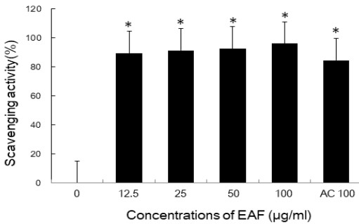
Fig. 1. DPPH radical scavenging activities of EAF extracts by various concentrations. DPPH radicals were generated as described in materials and methods. Ascorbic acid (AC 100 µM) was used as a positive control. The values are means ± SD of triplicate. *p<0.01 versus untreated group.
