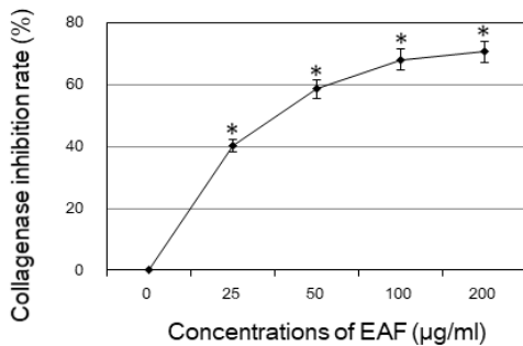
Fig. 2. Effects of EAF extracts on collagenase inhibition rate. Results are expressed as mean values ± S.D. of 3 replicates. *p<0.01 versus untreated group.
