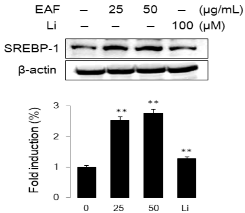
Fig. 5. Effect of EAF extracts on SREBP-1 expression in sebocytes. The cells were treated with EAF (25 or 50 \mu\text{g/ml} ) for 48 h. Cells lysates were analyzed by Western blot using SREBP-1 specific antibody. Data are representative of more than three independent experiment(mean \pm S.D). ** p < 0.01 vs. untreated group.
